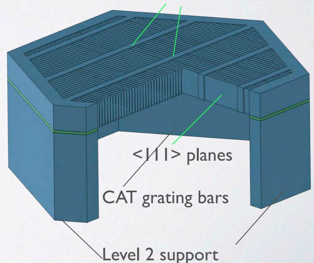
Critical-angle transmission gratings concept Credit: R. Heilmann
