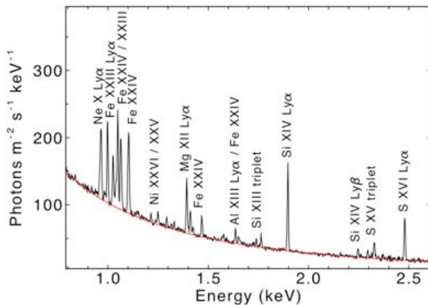
Figure 4: Close-up of a part of the spectrum of a bright cluster ( kT=2.5 \text{ keV} ) as seen by CRIS in 100 ks. Note the large number of lines from different elements.
