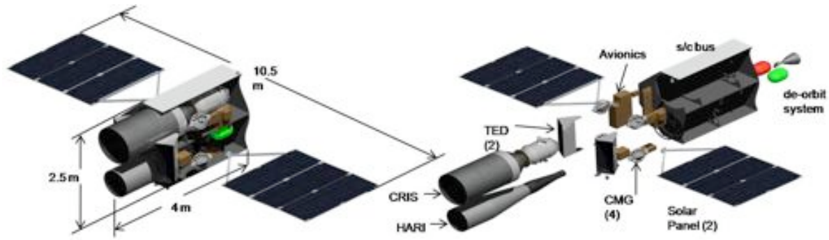
Figure 9: Xenia Spacecraft Concept
