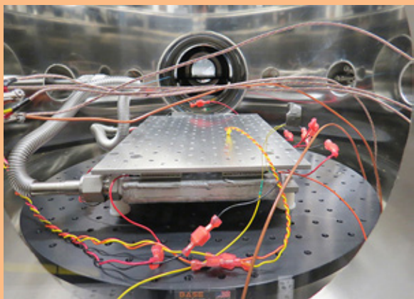
Fig. 7. Thermal cycling apparatus in our lab.
