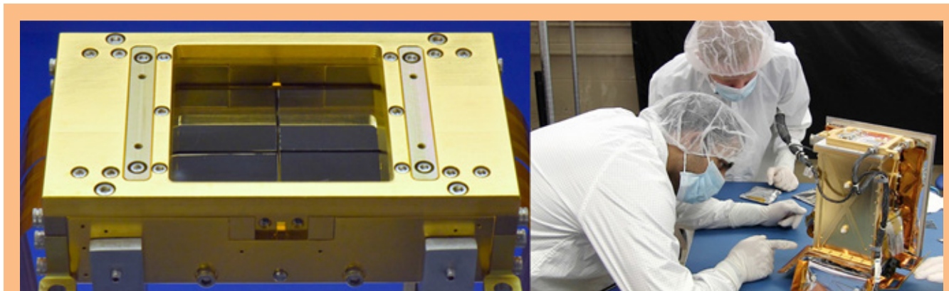
Fig. 10. Left: The REXIS DAM features four MIT/Lincoln CCDs, each with a directly deposited OBF. The total active area of the detectors is about 5\text{ cm} \times 5\text{ cm} . Right: Students preparing the REXIS instrument for environmental testing. We plan an Undergraduate Research Opportunities Program (UROP) project using REXIS engineering-model hardware to demonstrate that directly deposited OBF technology is at TRL 6. Images courtesy of MIT Lincoln Laboratory and MIT Space Sciences Laboratory.
