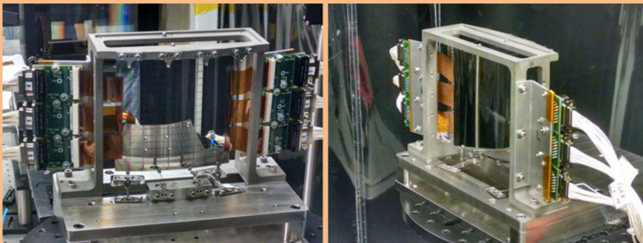
Fig. 4. Left: Front (concave side) view of a functional adjustable mirror mounted in its housing with electrical cables. Right: Back (convex side) view of the adjustable mirror in its housing. The ACF connections and the adapter boards can be seen.
