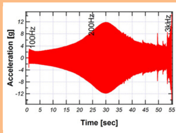
Fig. 10. Acceleration from vibration apparatus.
