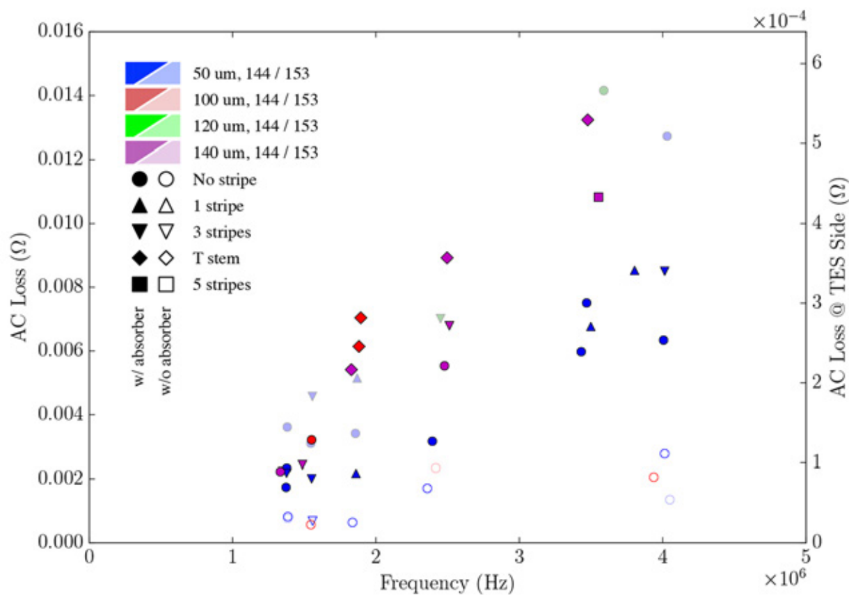
Fig. 5. Measured AC Loss (left axis) and AC Loss referred to the TES side of the transformer (right axis) as a function of AC-bias frequency for TESs of different sizes, different configurations of normal metal features, and with and without X-ray absorbers.
