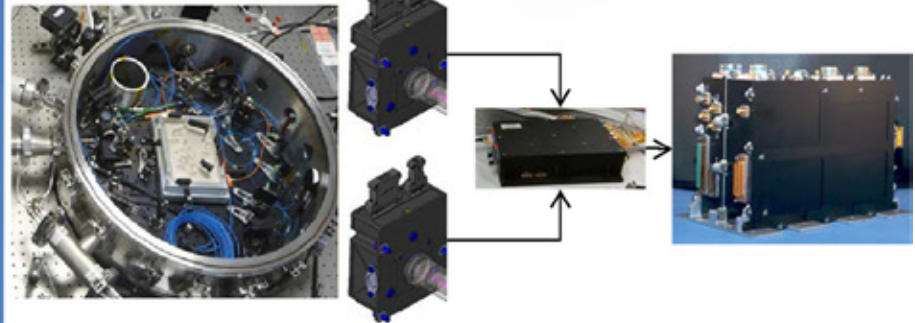
EM Hardware (QPD Photoreceivers, Pre-Amp, and Phasemeter) infused into the LISA Testbed
