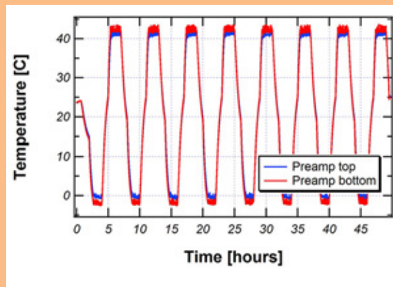
Fig. 8. Thermal levels in preamp tests.
