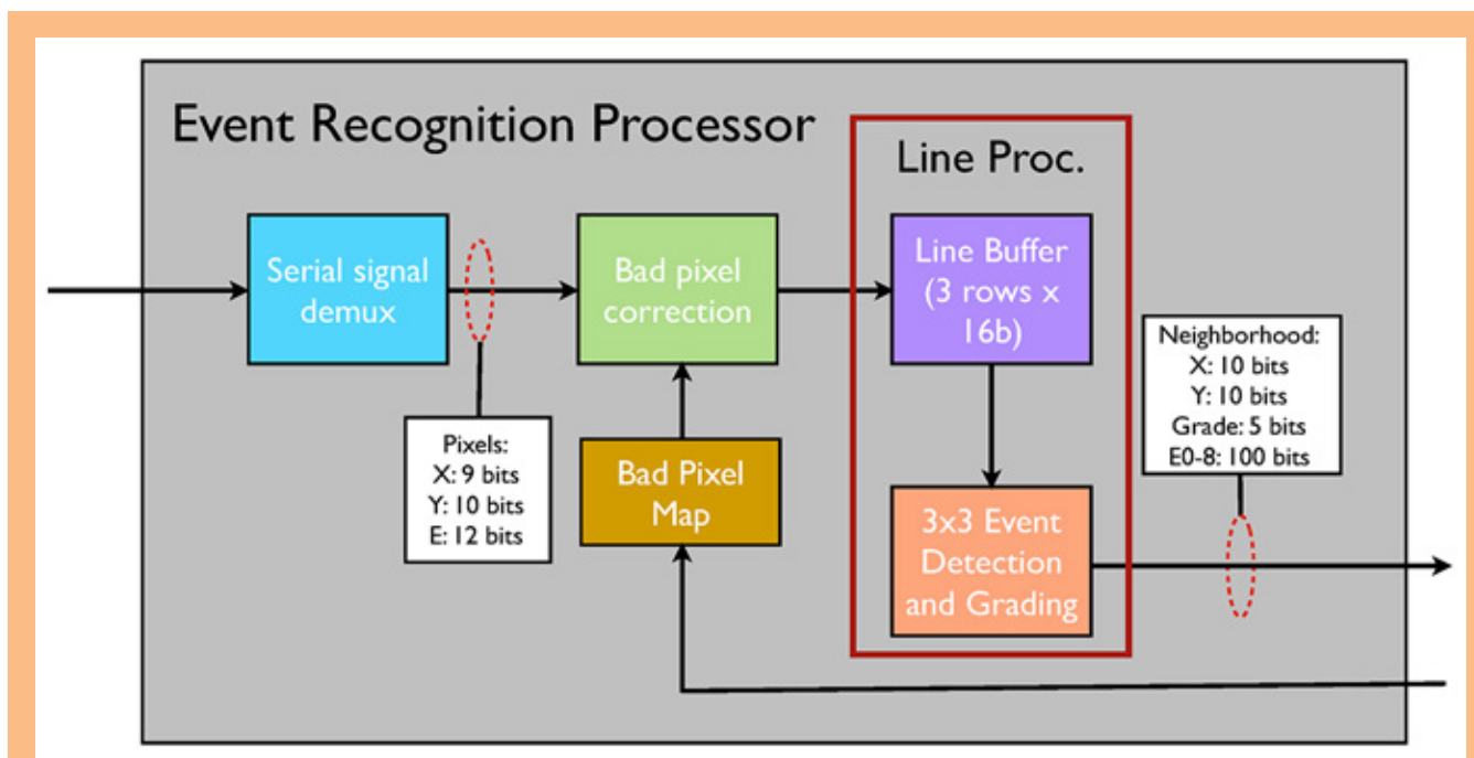
Fig. 3. A simplified block diagram of the ERP. High-speed serial digital data are demultiplexed and bad pixels are zeroed as needed. The data are then inserted into a three-line buffer in the Line Processor (LP) and scanned for valid X-ray events using a sliding 3 \times 3 pixel window. Event grades are encoded based on a simple comparator with a settable threshold. Output data are 3 \times 3 “neighborhoods” centered on candidate X-ray events. Bit assignments shown are nominal.
